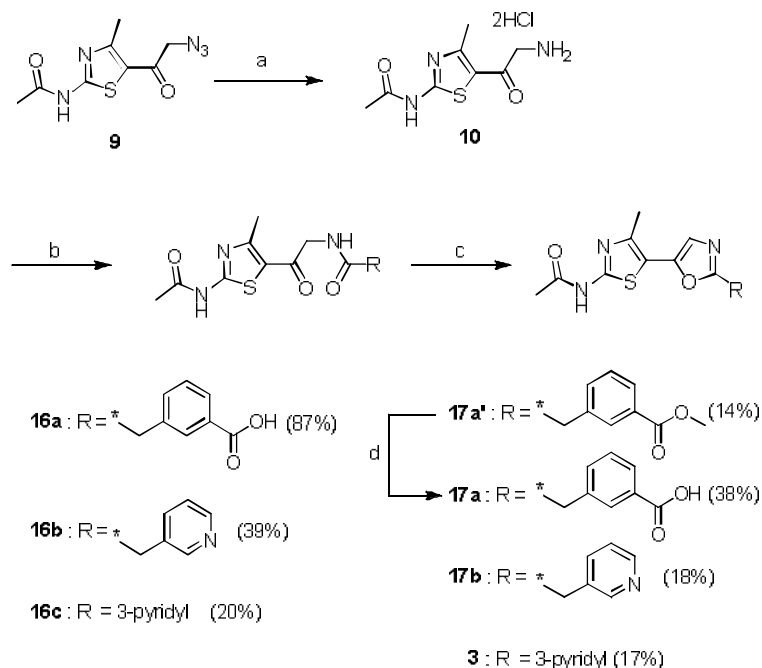
Scheme 3. Reagents and conditions: (a) \text{H}_2 , 10% Pd/C, c.HCl, MeOH, rt, 18 h, 75%; (b) R-COOH, PyBOP ® , Et 3 N, DMF, rt, or R-COCl, Et 3 N, THF-CHCl 3 , rt; (c) POCl 3 , reflux, or Burgess reagent, THF, 80 °C; (d) aq. KOH, THF-MeOH, 60 °C, 5 h, 38%.
