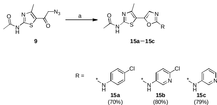
Scheme 2. Reagents and conditions: (a) R-NCS, PPh 3 , 1,4-dioxane, 100 °C.
