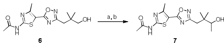
Scheme 9. Reagents and conditions: (a) PCC, CHCl 3 -THF, 6 h, rt, (b) MeMgBr, THF, rt, 3 h, 15% (2 steps).
