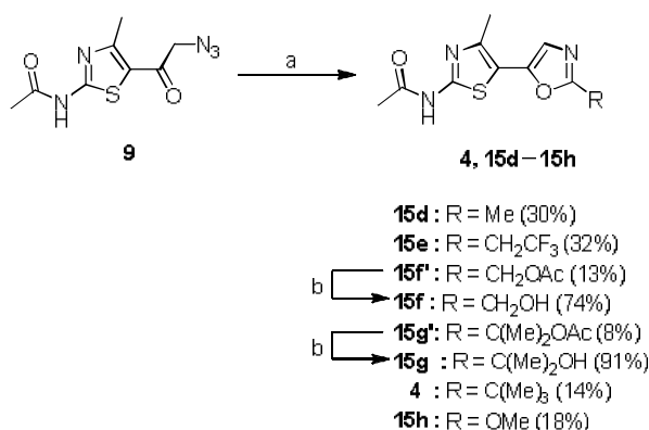
Scheme 5. Reagents and conditions: (a) R-COCl, PPh 3 , THF or 1,4-dioxane, rt; (b) aq. KOH, THF-MeOH, 60 °C.
