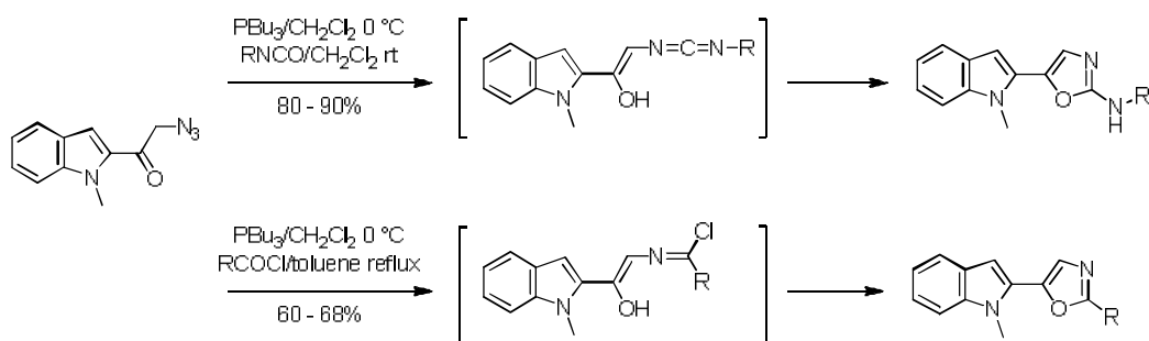
Scheme 11. Known approach for oxazoles having various substitutions.
