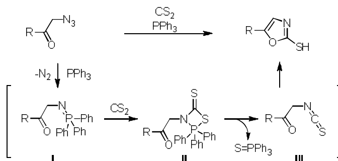
Scheme 12. plausible mechanism of iminophosphorane-mediated 2-sulfanyloxazole formation.
