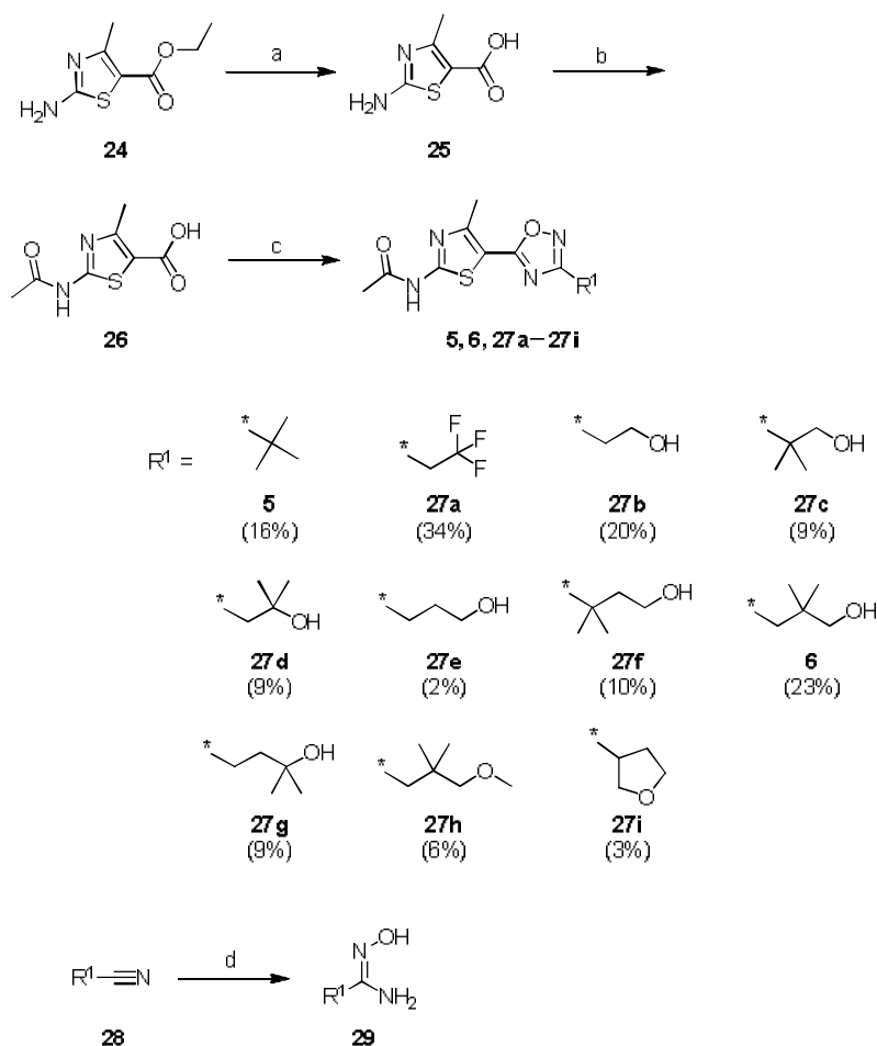
Scheme 8. Reagents and conditions: (a) aq. NaOH, EtOH, rt, 26 h, 97%; (b) acetyl chloride, pyridine, THF, rt, 21 h, 91%; (c) 29 , EDC·HCl, HOBT·H 2 O, DMF, rt then 100 °C; (d) 50% hydroxylamine solution, EtOH, reflux.
