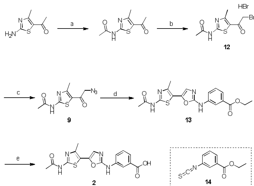
Scheme 1. Reagents and conditions: (a) acetyl chloride, pyridine, THF-CHCl 3 , rt, 72 h, 92%; (b) bromine, 1,4-dioxane, rt, 14 h, 50%; (c) NaN 3 , Et 3 N, MeOH, rt, 3 h, 90%; (d) 14 , PPh 3 , 1,4-dioxane, 100 °C, 1 h, 79%; (e) aq. KOH, THF-MeOH, 60 °C, 3 h, 51%.
