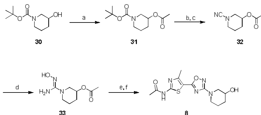
Scheme 10. Reagents and conditions: (a) acetyl chloride, pyridine, rt, 4 h; (b) 4 M HCl-AcOEt, AcOEt, rt, 24 h; (c) cyanogen bromide, K 2 CO 3 , CH 3 CN, rt, 4 h, 79% (3 steps); (d) 50% hydroxylamine solution, EtOH, reflux, 1 h; (e) 26 , EDC·HCl, HOBT·H 2 O, DMF, rt, 15 h, then 100 °C, 3 h; (f) 2 M NaOH, THF-EtOH, rt, 15 h, 10% (3 steps).
