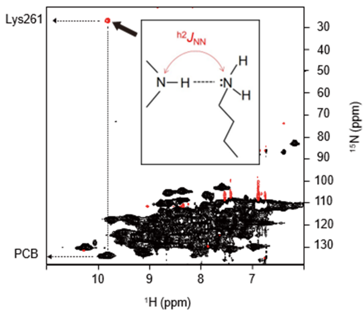
図5 HNN-COSY
